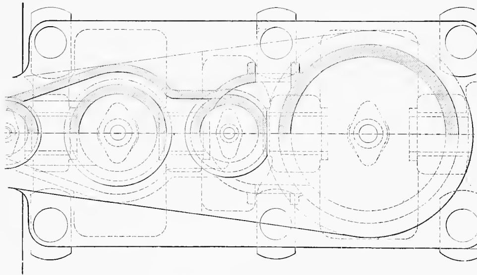
SECTION PLAN OF CYLINDERS.
